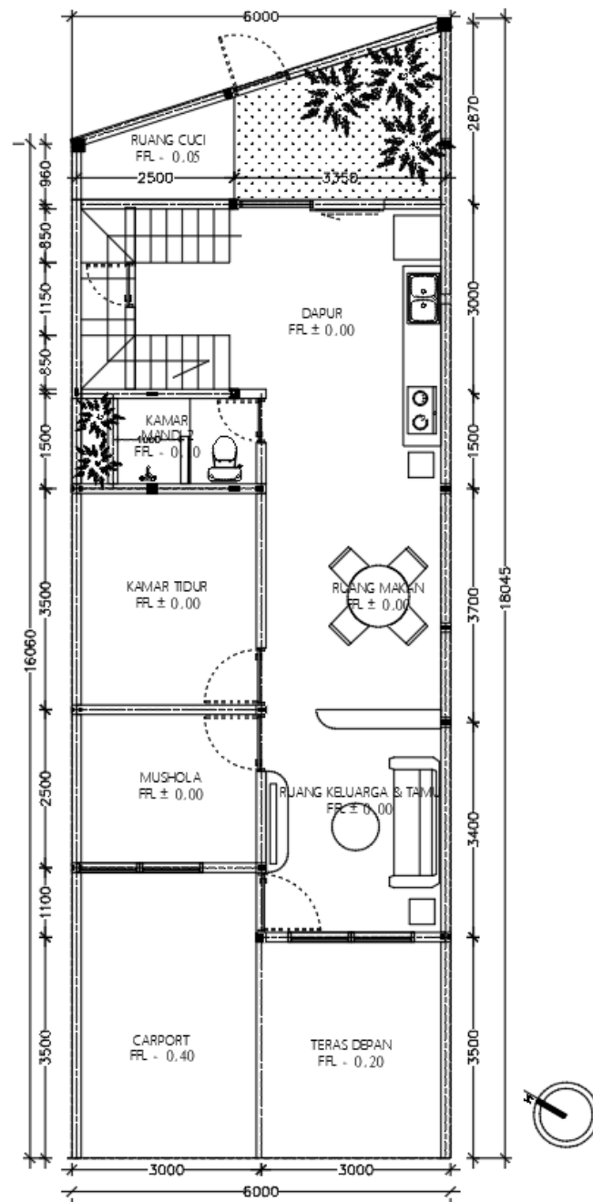
DENAH LANTAI 1
