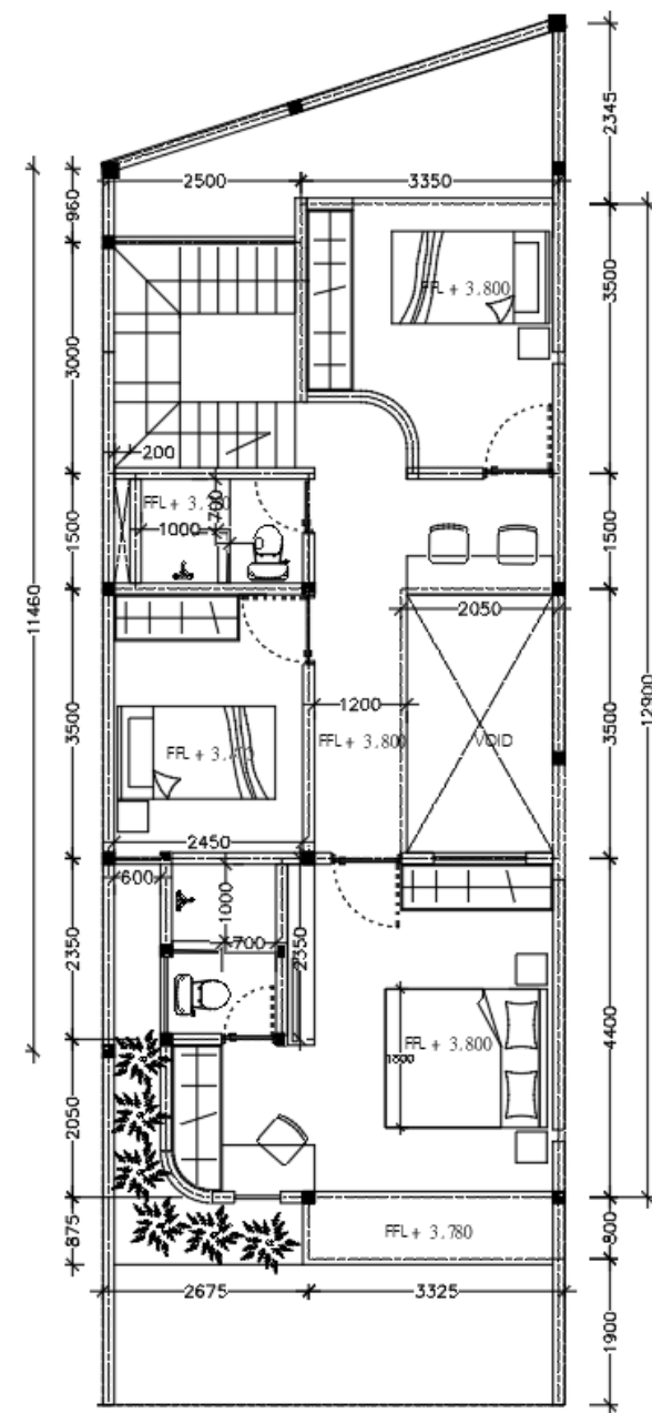
DENAH LANTAI 2
